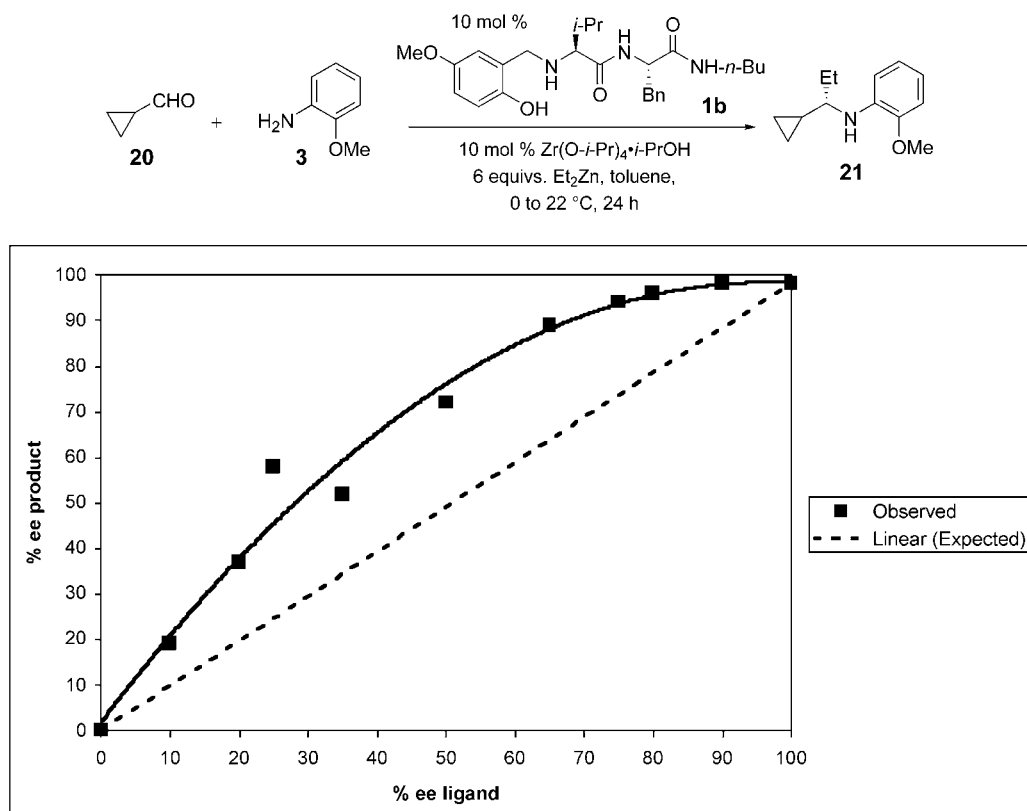
Figure 1. Plot of % ee product vs. % ee ligand for enantioselective synthesis of 21 .
