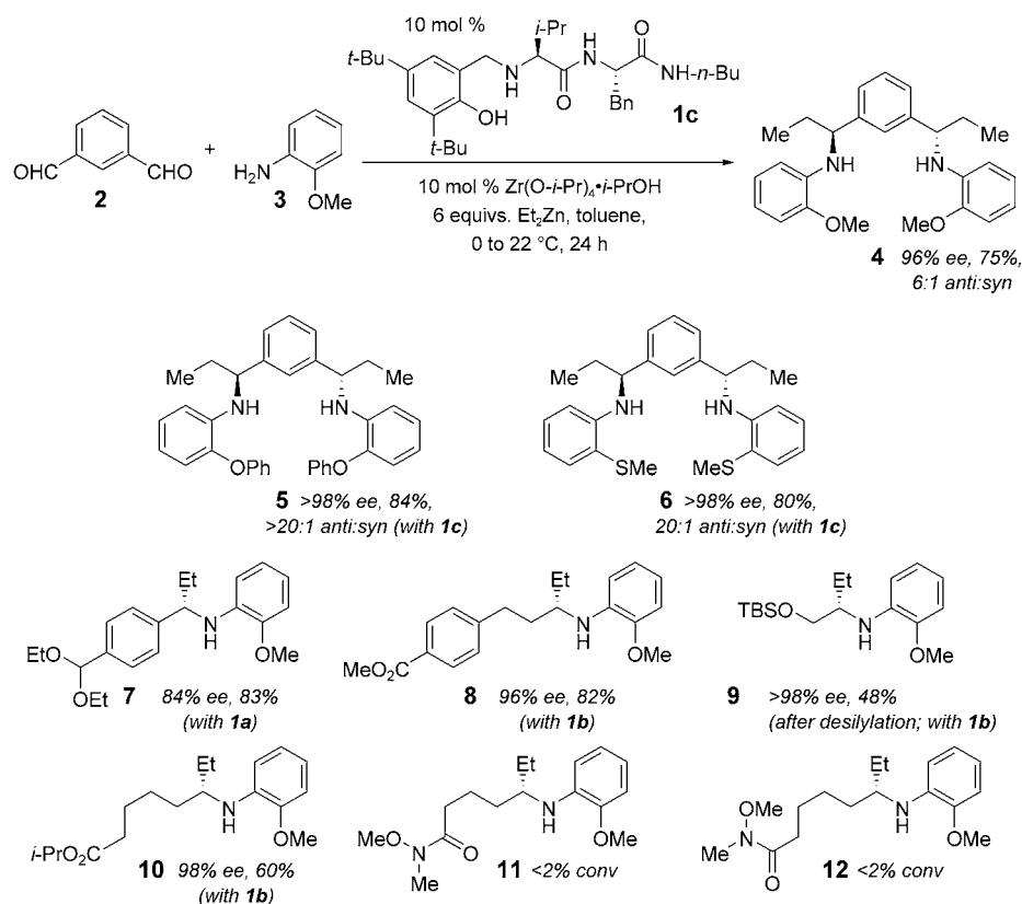
Scheme 2. New examples of Zr-catalyzed enantioselective imine alkylations.
