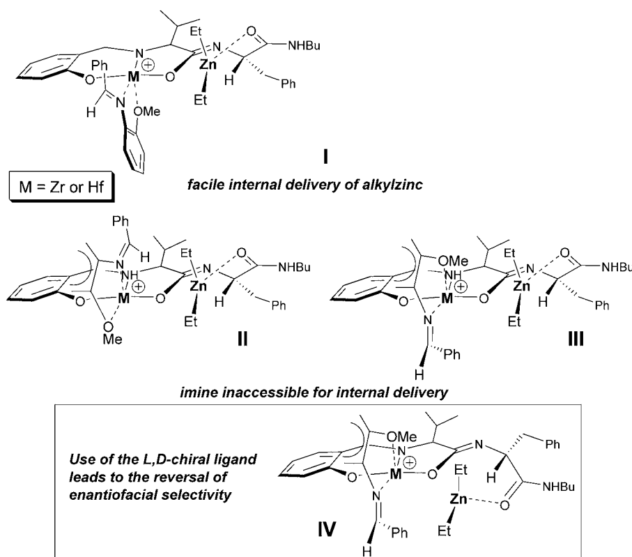
Scheme 3. Proposed models for Zr-catalyzed asymmetric alkylation of imines.
