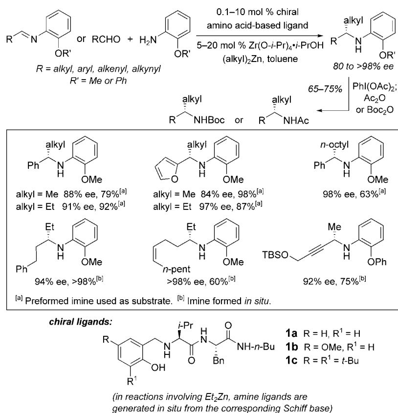
Scheme 1. Zr-catalyzed enantioselective synthesis of amines and derivatives.
